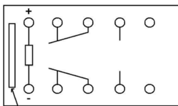
MONOSTABLE
