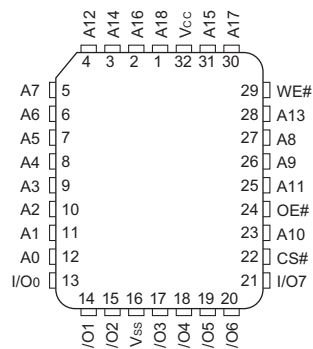
32 CLCC
