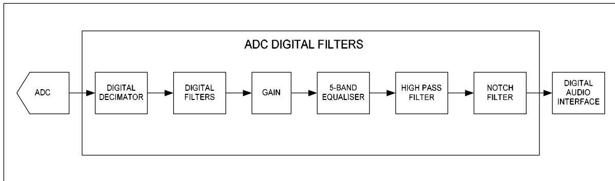
Figure 9 ADC Digital Filter Path
