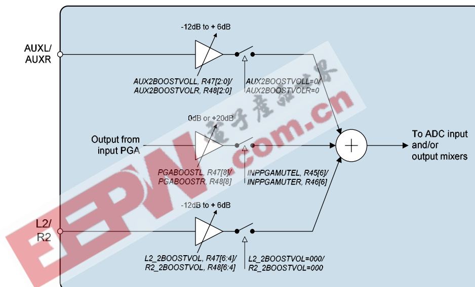
Figure 7 Input Boost Stage
