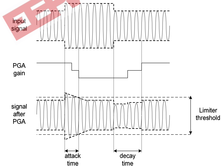
Figure 10 Input Peak Limiter Operation
