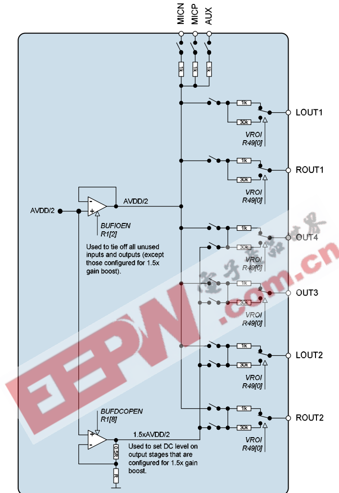
Figure 22 Unused Input/Output Pin Tie-off Buffers
