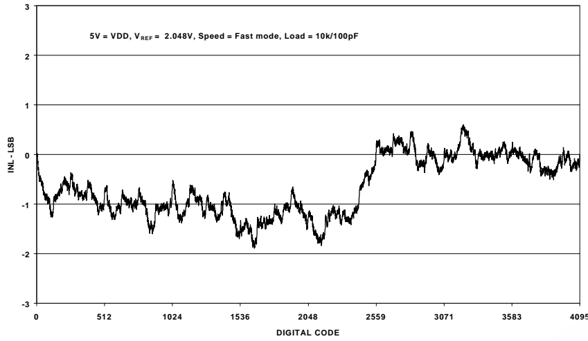
Figure 2 Integral Non-Linearity
