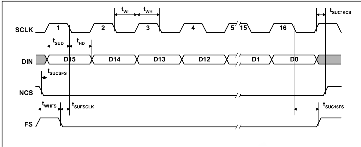
Figure 1 Timing Diagram
