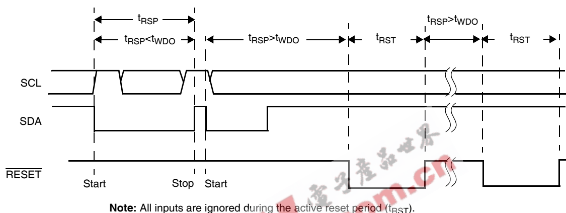
Figure 3. Watchdog Restart/Time Out
