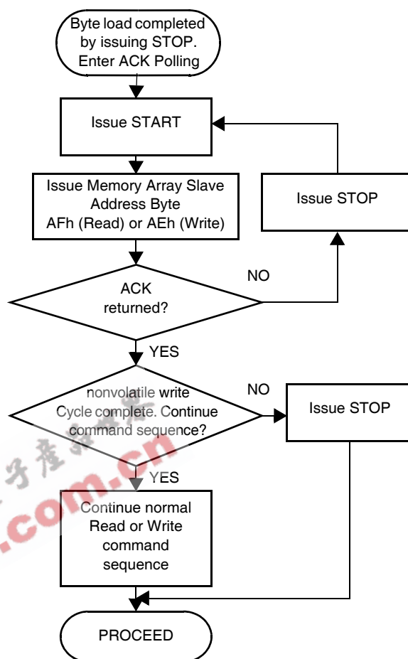
Figure 15. Acknowledge Polling Sequence
