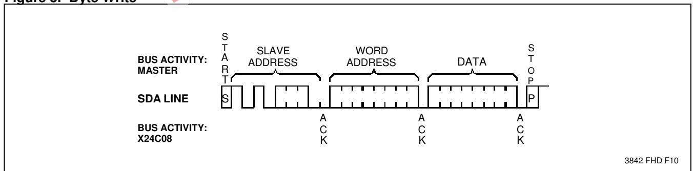
Figure 5. Byte Write
