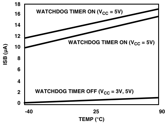
FIGURE 15. V CC SUPPLY CURRENT VS. TEMPERATURE (I SB )
