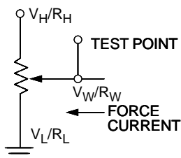
Test Circuit #2
