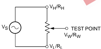
Test Circuit #1
