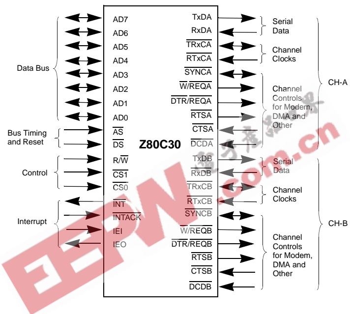
Figure 5. Z80C30 Pin Functions
