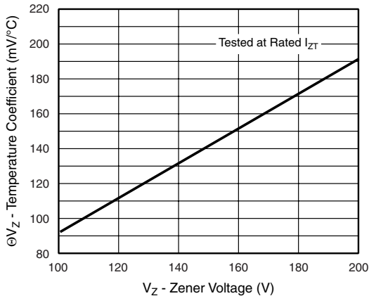
Figure 5. Typical Temperature Coefficients
