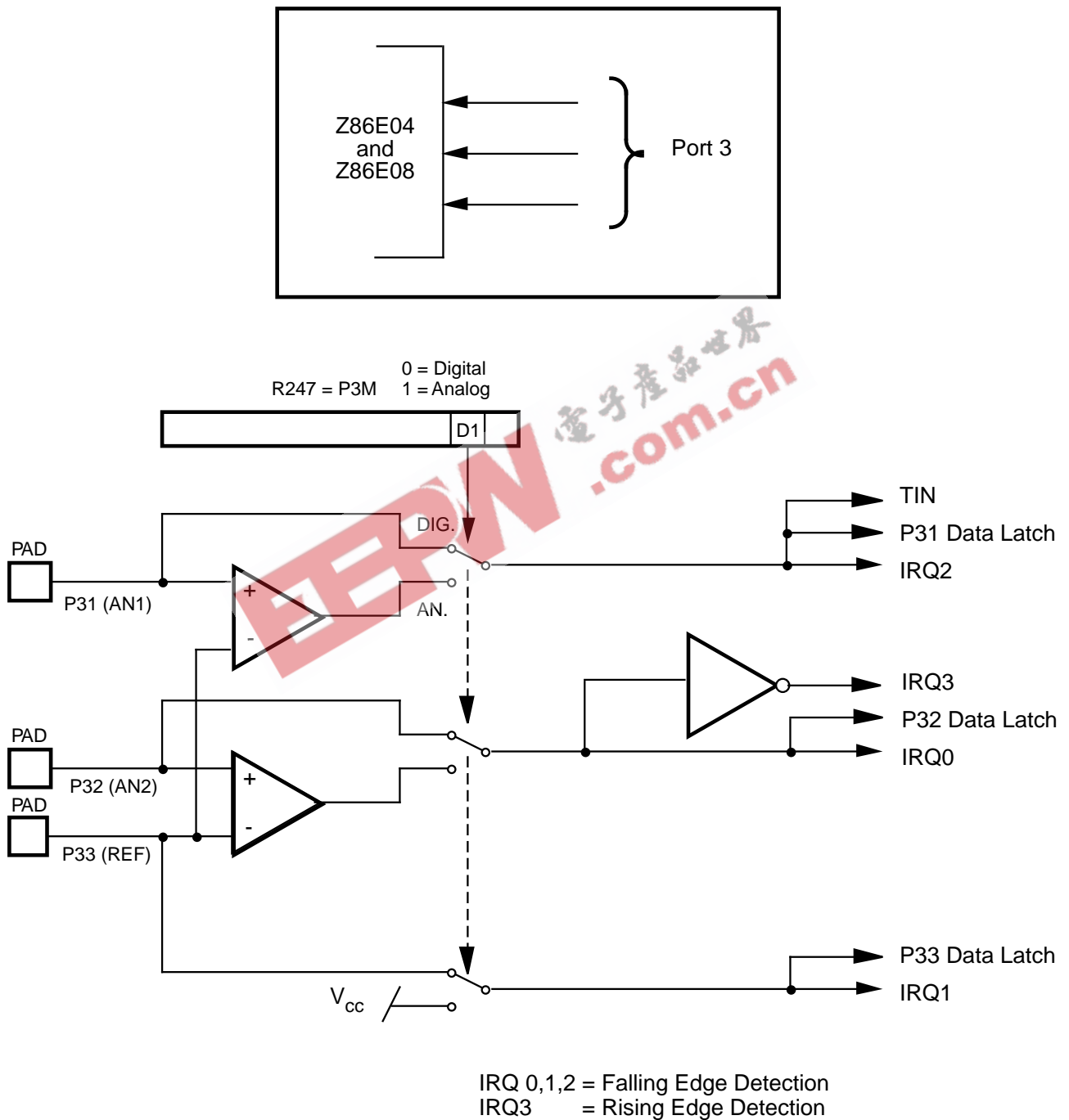
Figure 9. Port 3 Configuration
