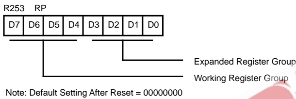
Figure 64. Register Pointer (F DH : Read/Write)
