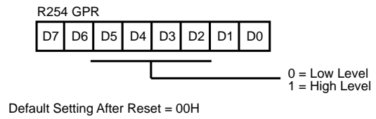
Figure 65. General-Purpose Register (F EH : Read/Write)
