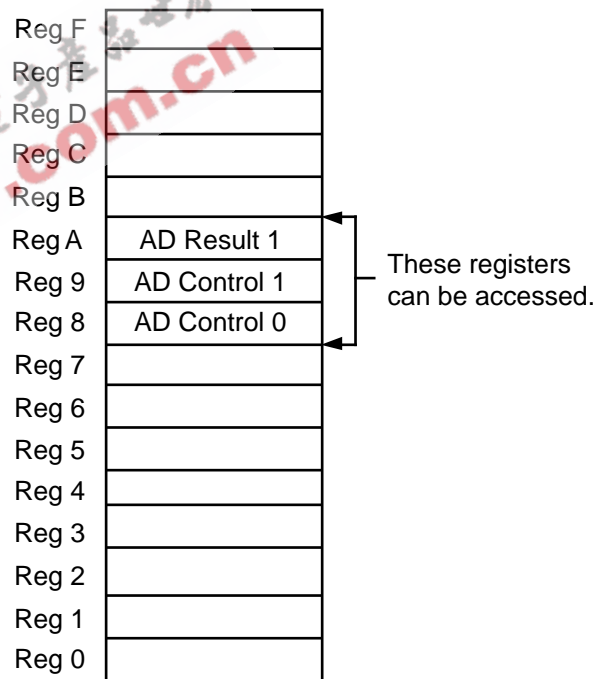
Figure 26. Bank C
