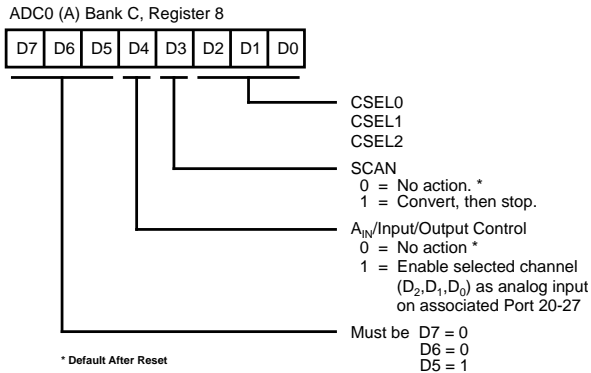
Figure 23. ADC Control Register 0 (Read/Write)
