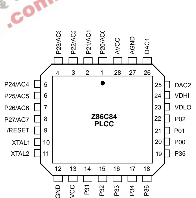
Figure 5. Z86C84 28-Pin PLCC Pin Configuration
