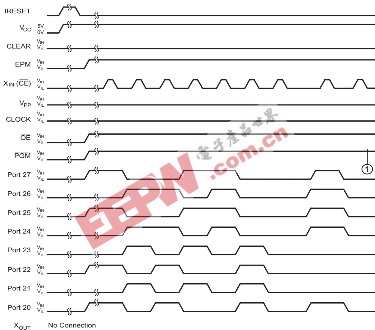
Figure 6. Unlock Sequence
