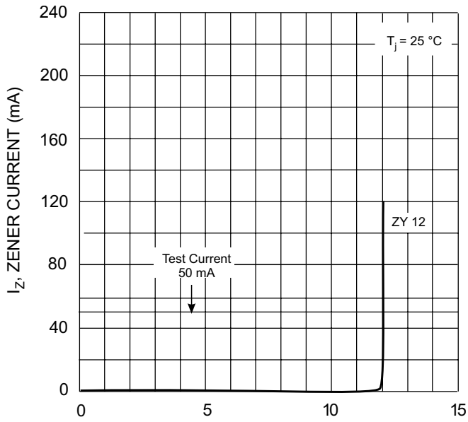
Fig. 1 Zener Breakdown Characteristics
