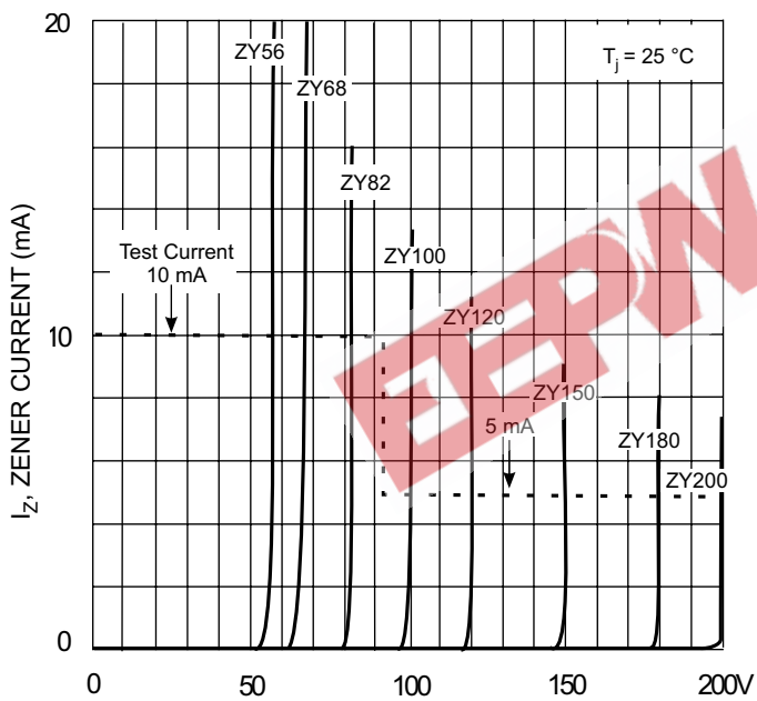
Fig. 3 Zener Breakdown Characteristics
