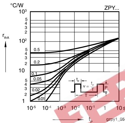
Figure 2. Pulse Thermal Resistance vs. Pulse Duration
