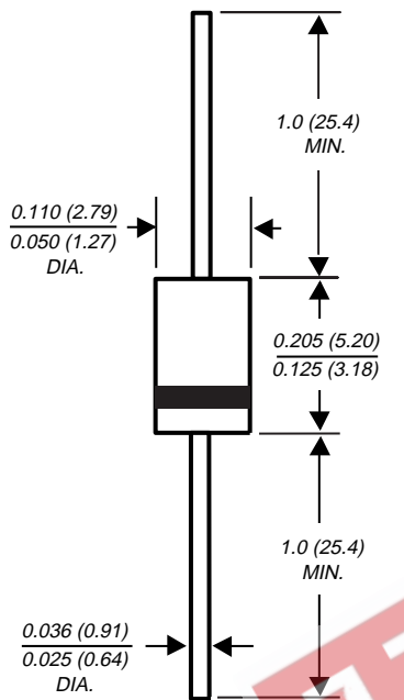
DO-204AM
