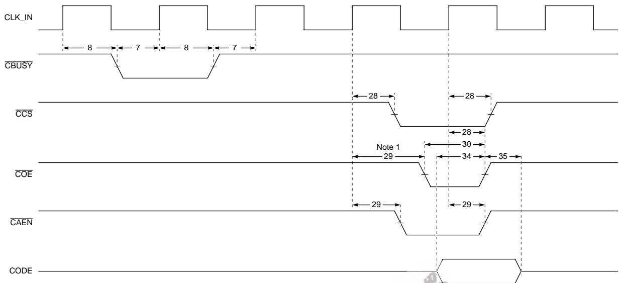
Figure 46. Master Mode Compressed Data Transfer Timing (Decoding)
