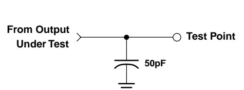
Figure 35. Normal AC Test Load
